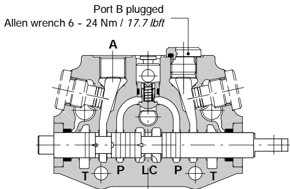
P-A-T closed, with flow through line (LC) open
