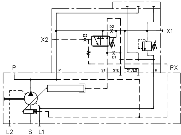
Coding Pb
