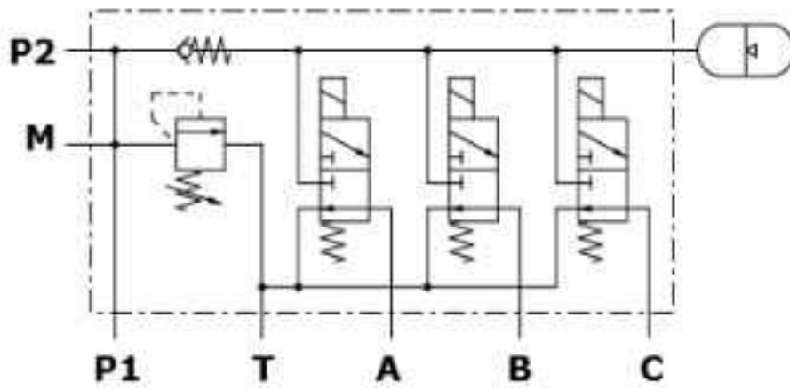
Hydraulic circuit
