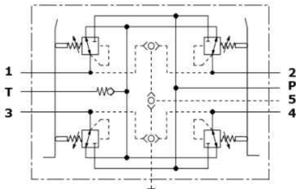
Hydraulic circuit
