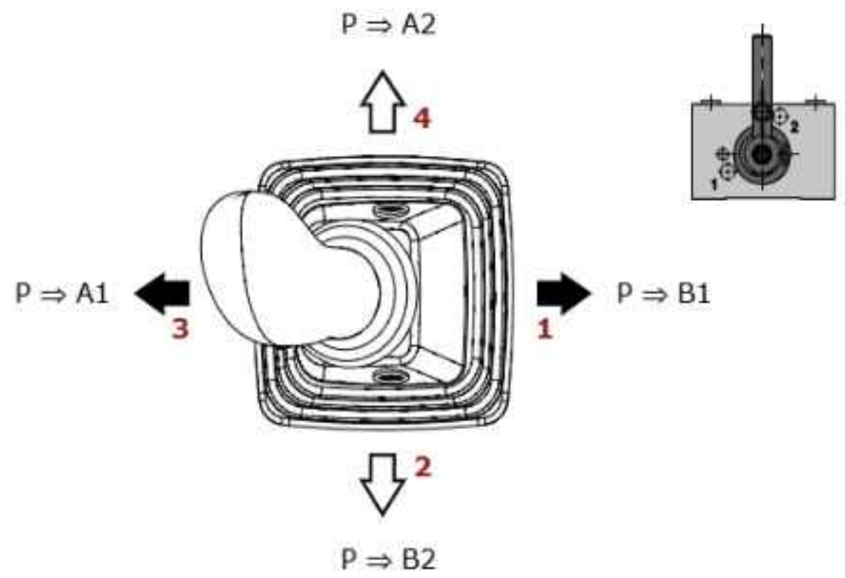
Diverter valve in position 2 Mini-excavator configuration
