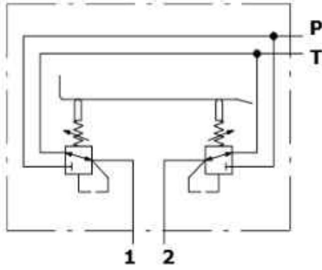
Hydraulic circuit
