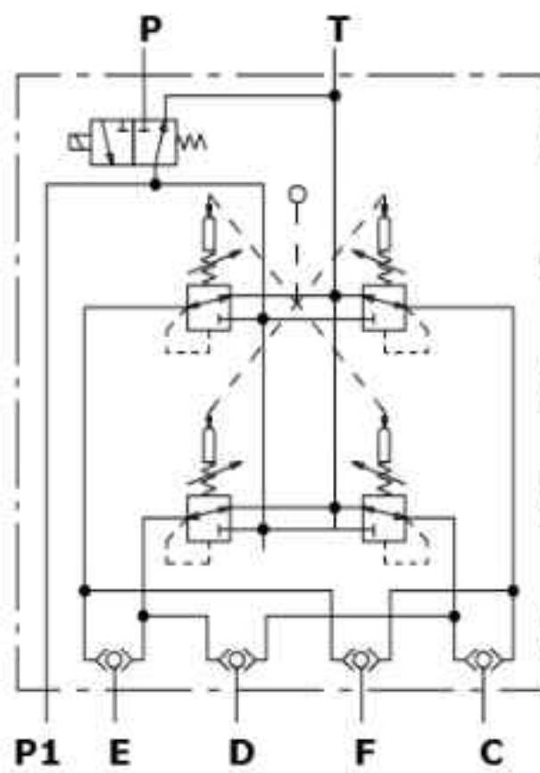
Hydraulic circuit
