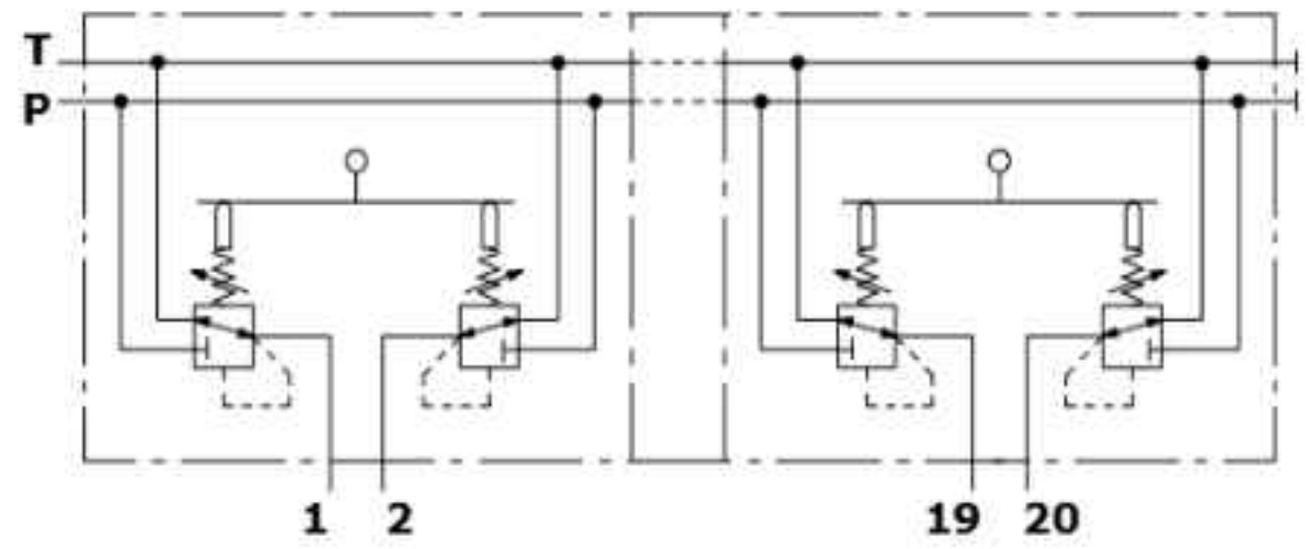
Hydraulic circuit
