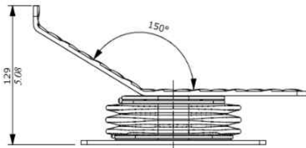
Right pedal 01B3R type
