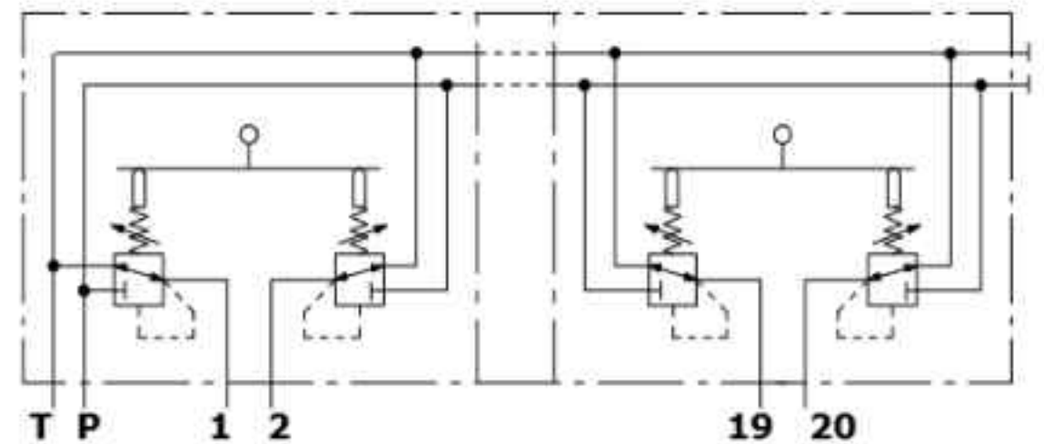
Hydraulic circuit
