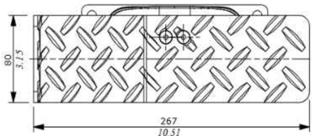
Left pedal 01B3L type
