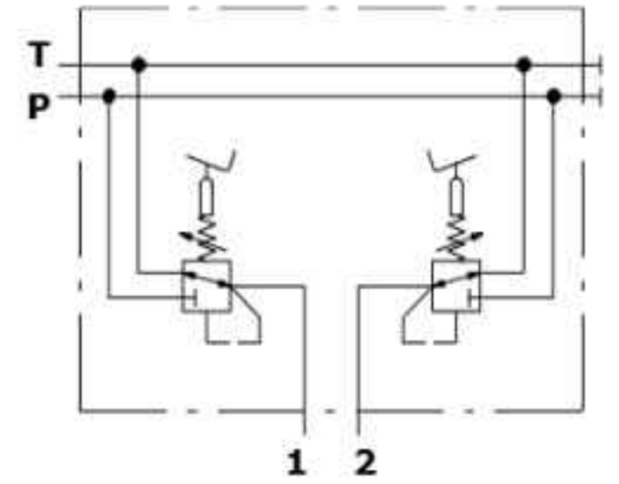
Hydraulic circuit
