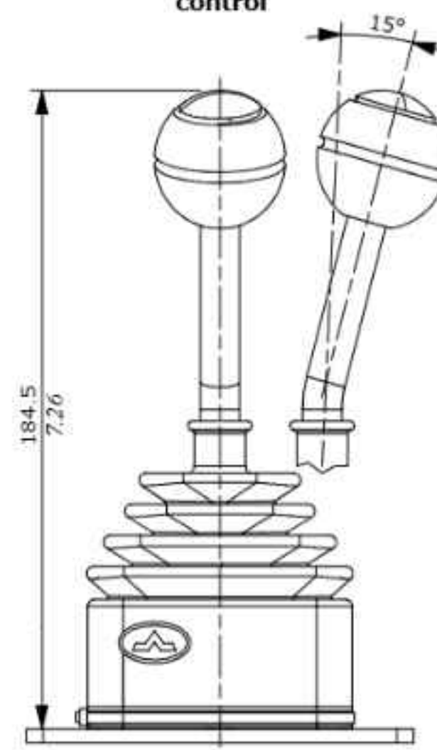
03E3 control
