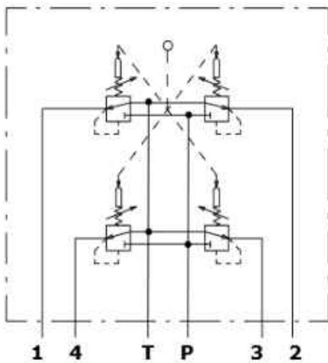
Hydraulic circuit
