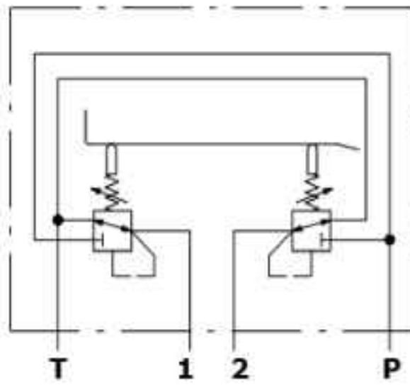
Hydraulic circuit
