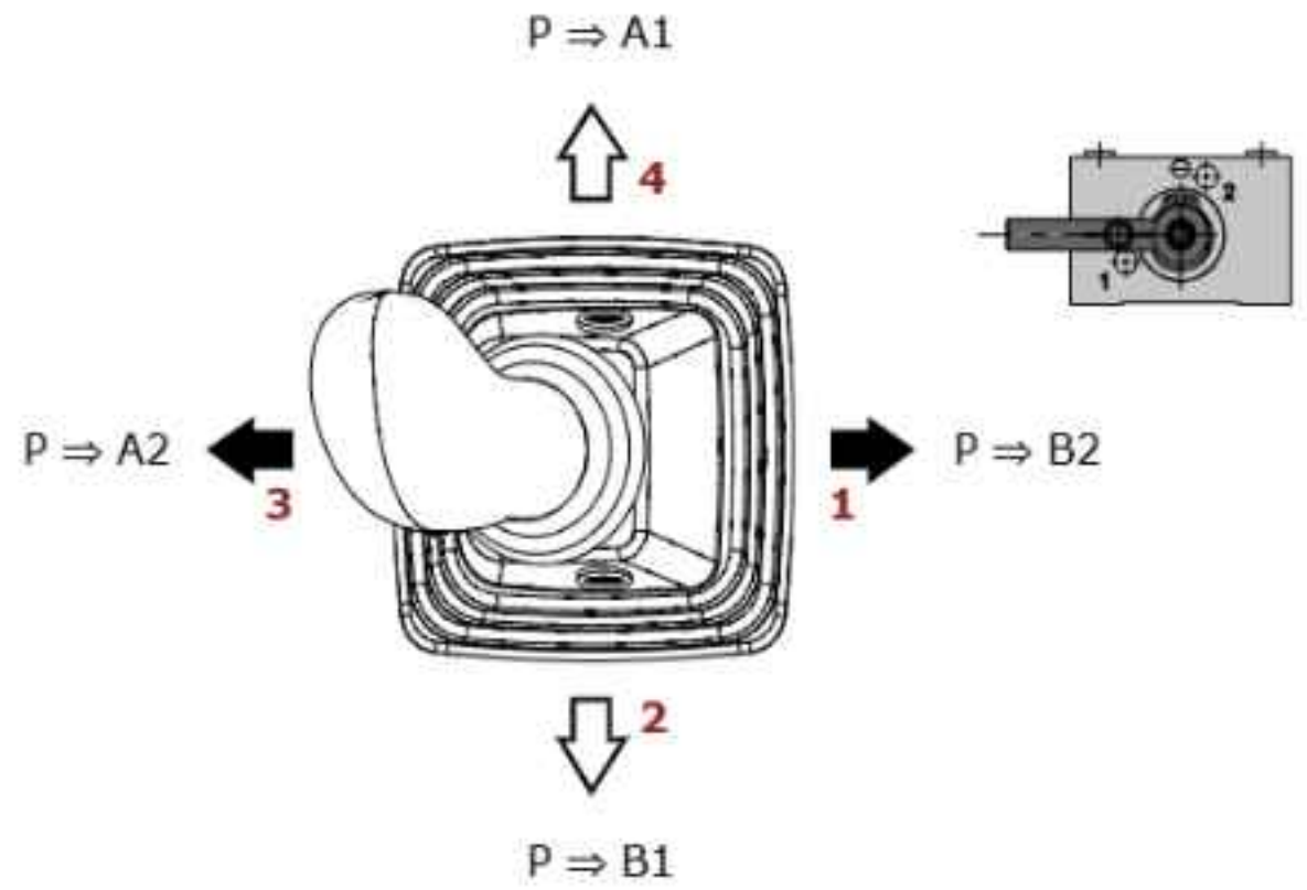
Diverter valve in position 1 Backhoe configuration
