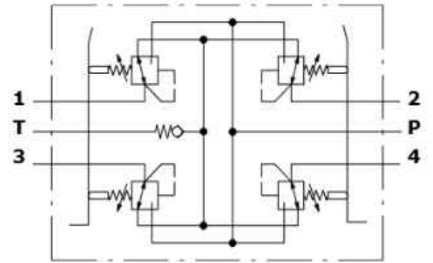
Hydraulic circuit
