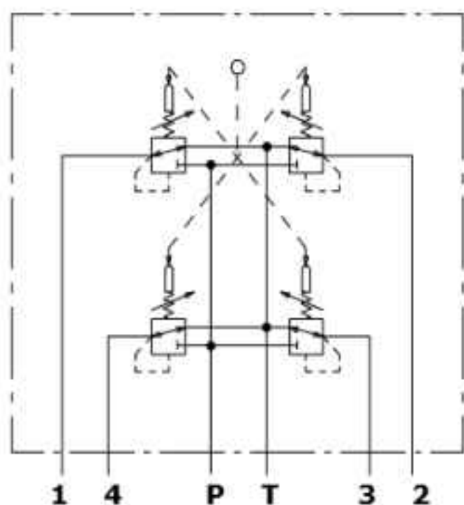
Hydraulic circuit
