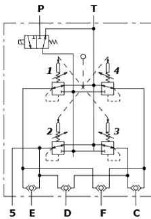
Hydraulic circuit
