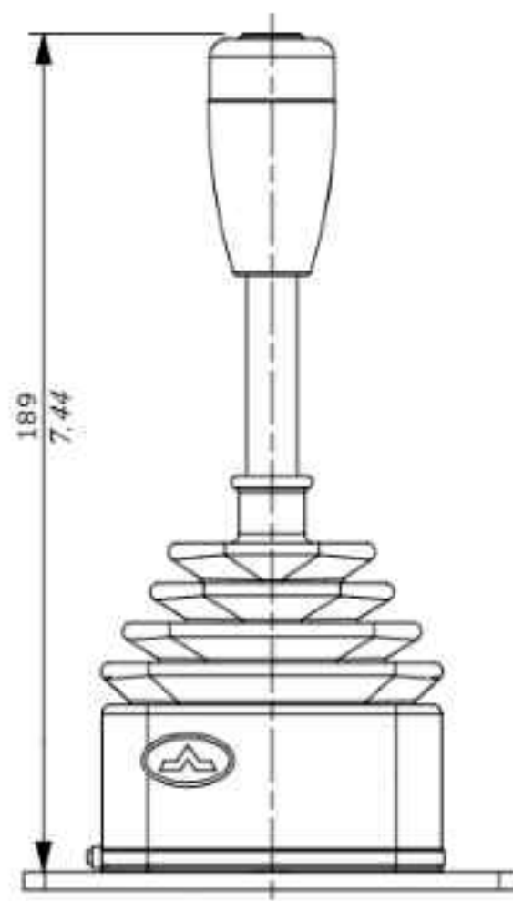
03JL3 control
