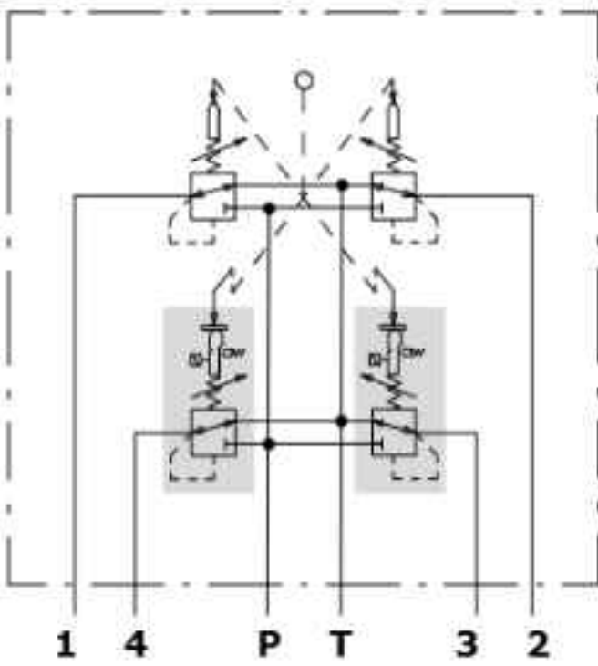
hydraulic circuit Example detent on working ports 3 e 4
