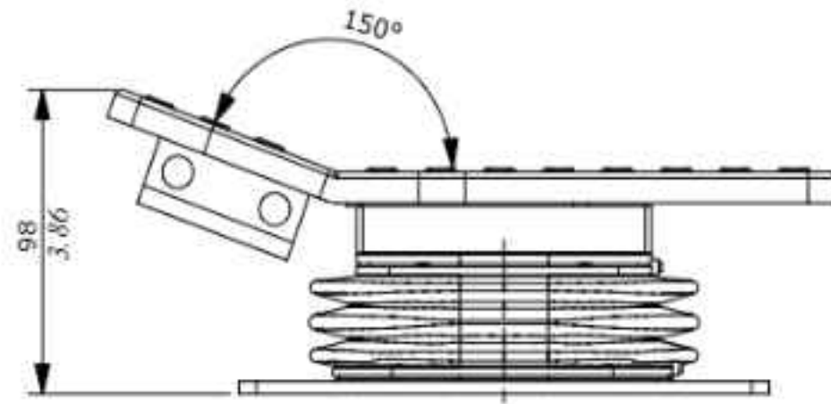
0101P assembly on the right
