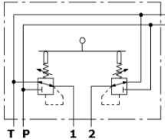
Hydraulic circuit
